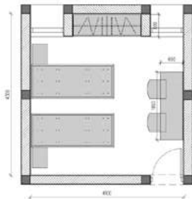
Double room with different entry door
