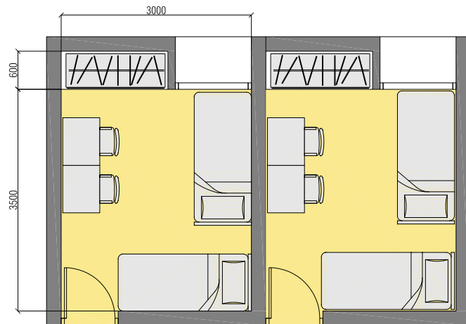
Architect's drawing to show how a single room could be configured for double occupancy
