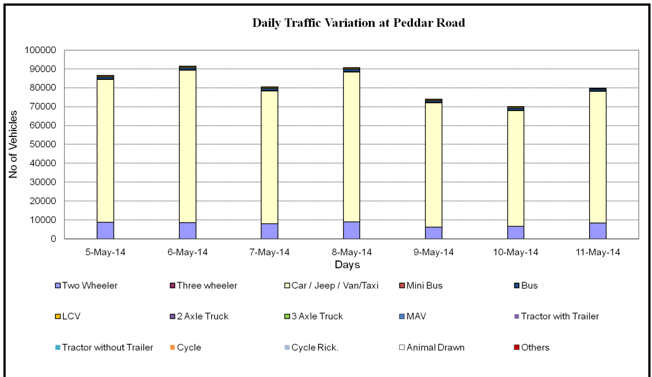
Figure 2.16: Daily Traffic Variation at Peddar Road
