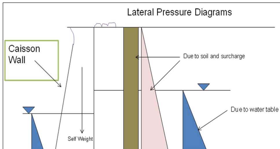
Forces for Analysis
