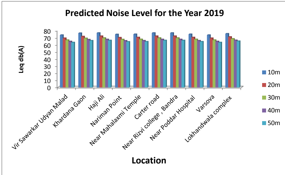
Figure 5.2: Noise prediction for the year 2019
