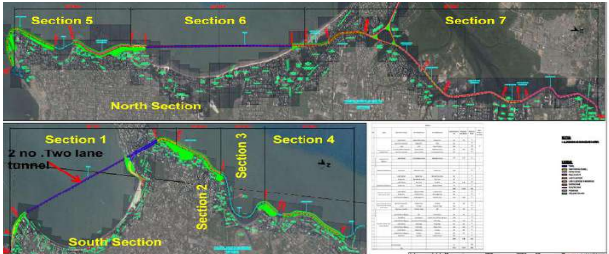
Alignment Option – 6
