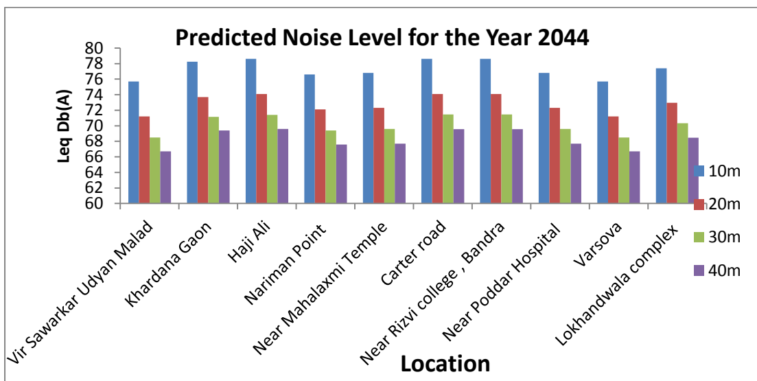
Figure 5.7: Noise prediction for the year 2044
