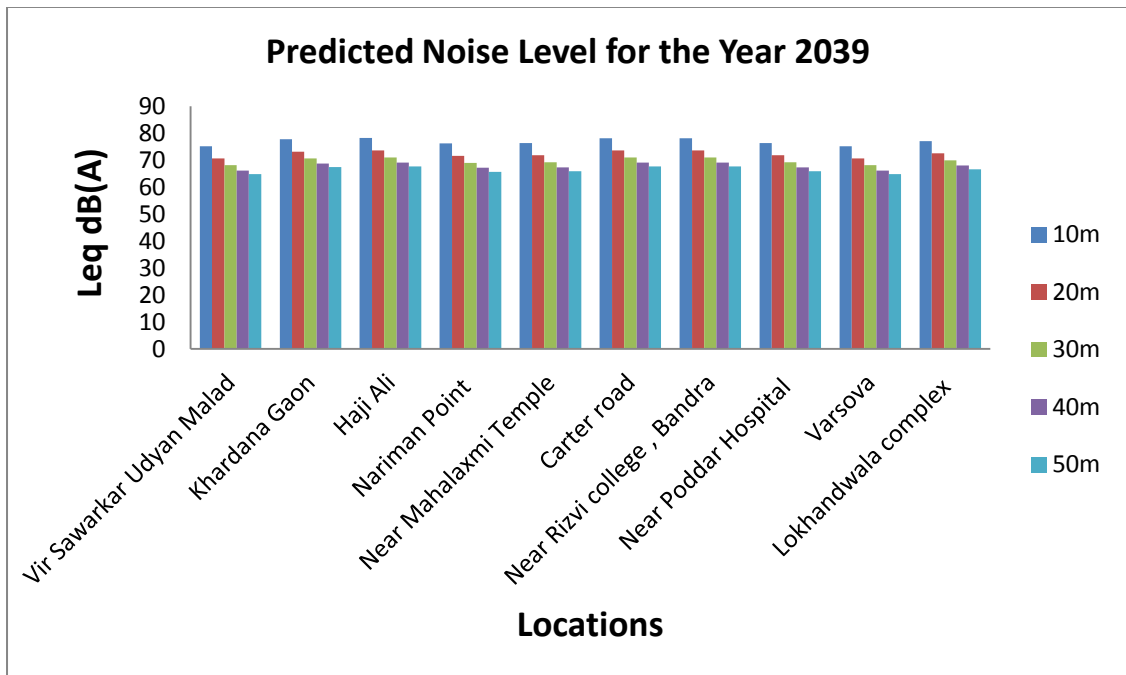
Figure 5.6: Noise prediction for the year 2039
