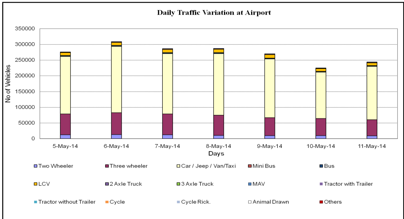
Figure 2.14: Daily Traffic Variation at Airport
