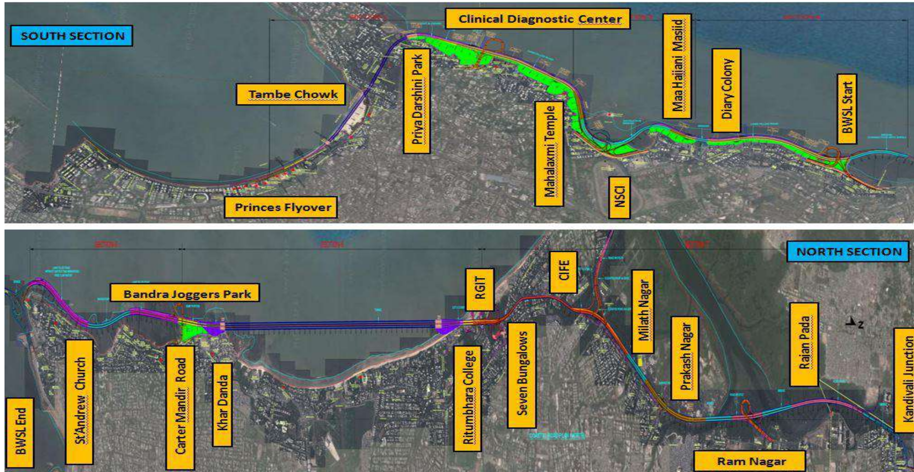
Figure 3.1: Alignment of Mumbai Coastal Road Project (Option 7)
