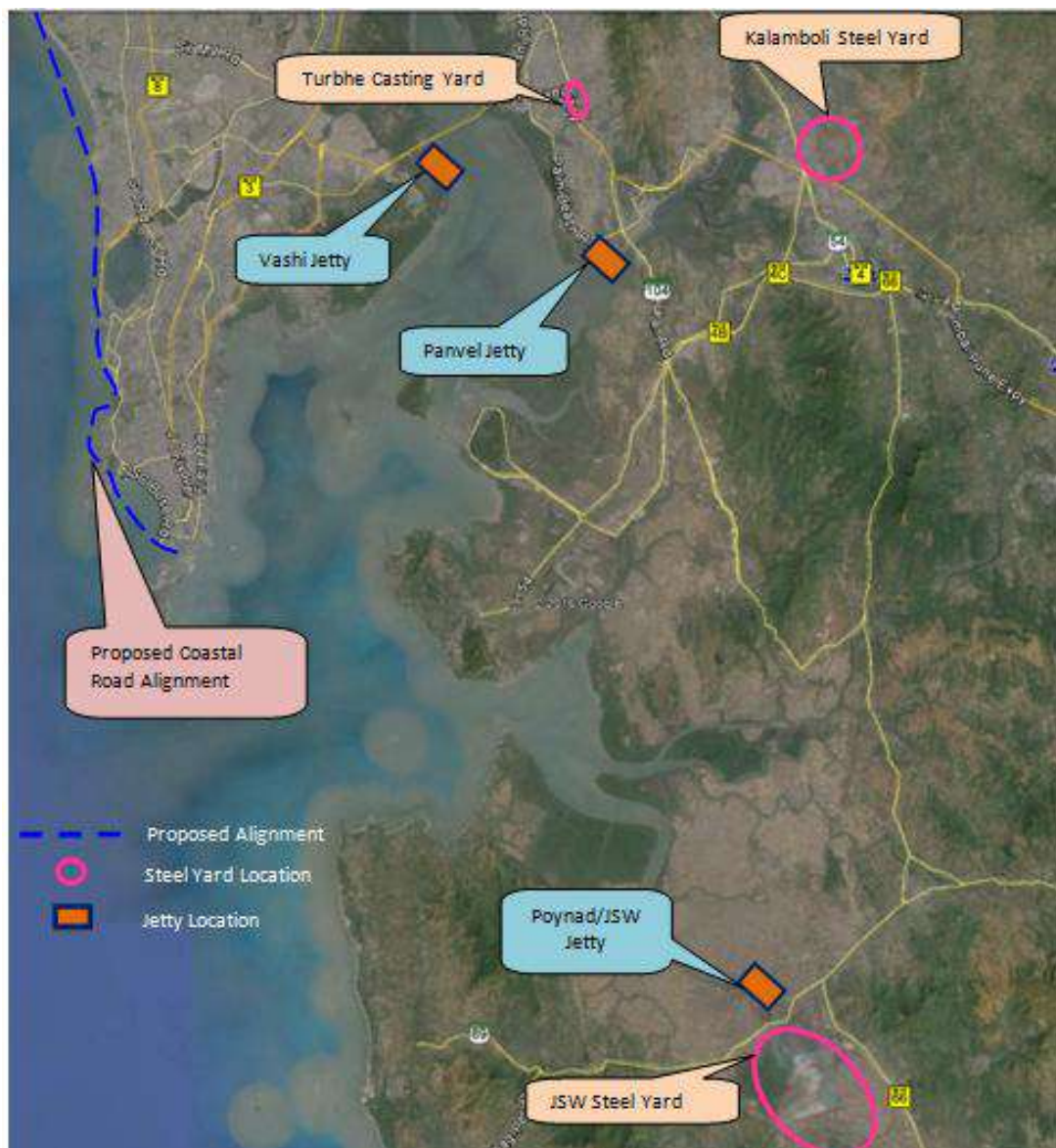
Figure 2.30: Steel Yard Locations
