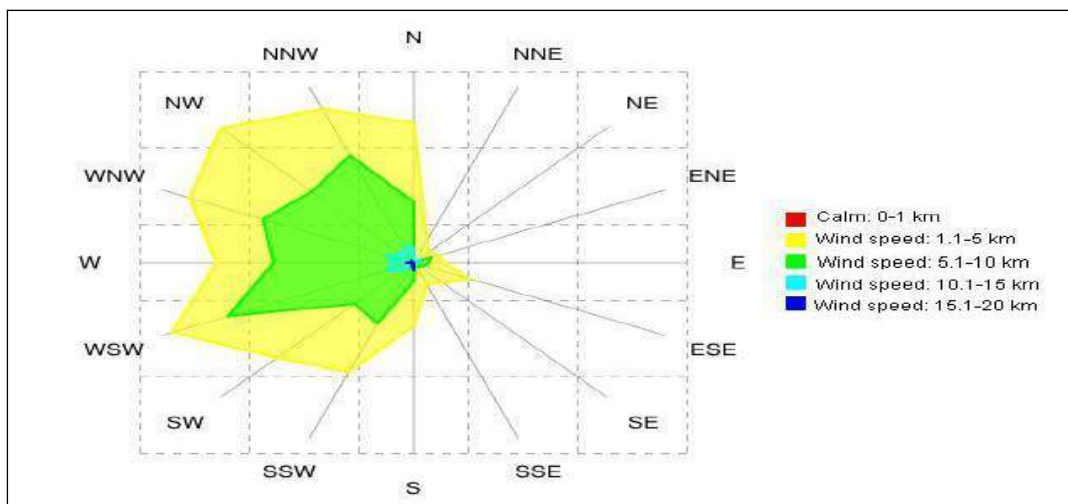
Figure 4.5: WIND ROSE Diagram
