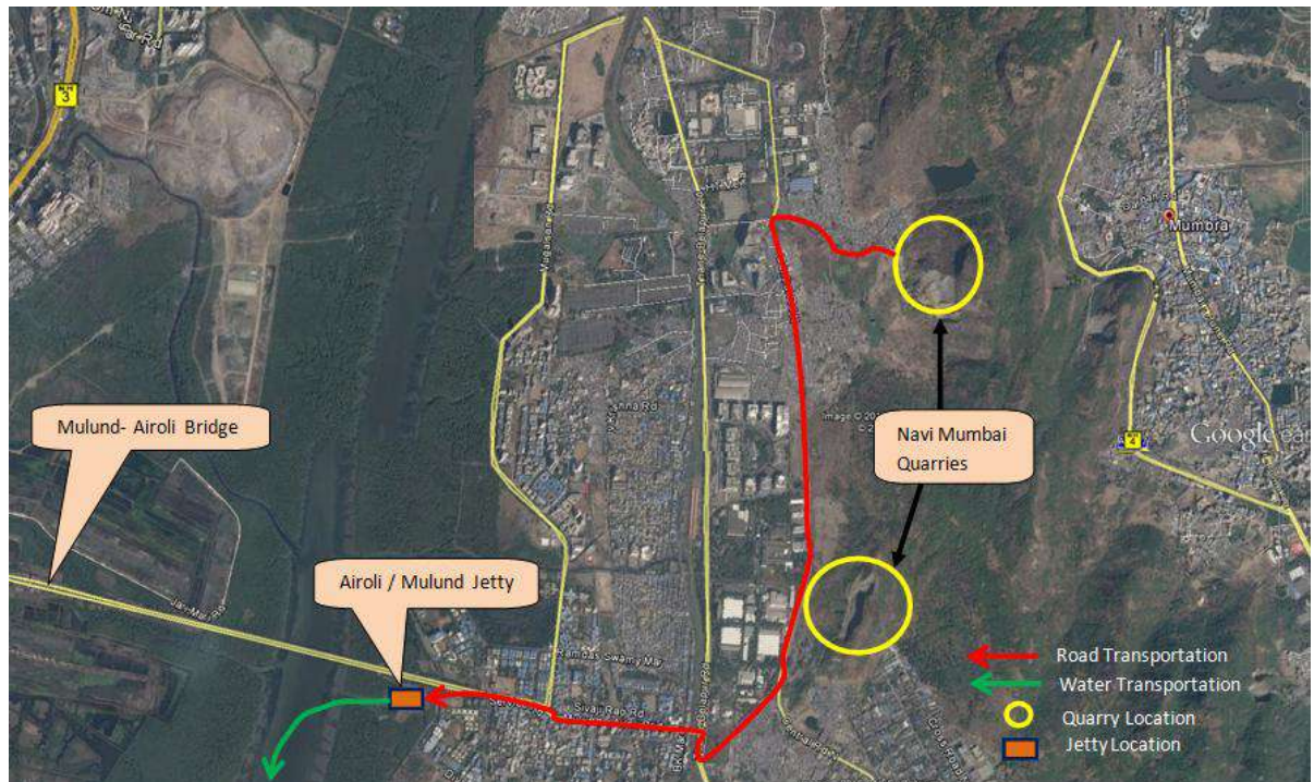
Figure 2.27: Transportation Plan from Navi Mumbai Quarry
