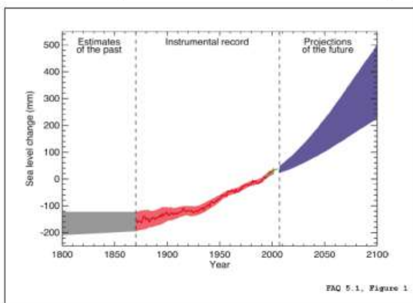
Figure 2.22: Level Changes – Past, Present and Future (Ref: Unnikrishanan A. S and Shankar. D NIO, Goa)
