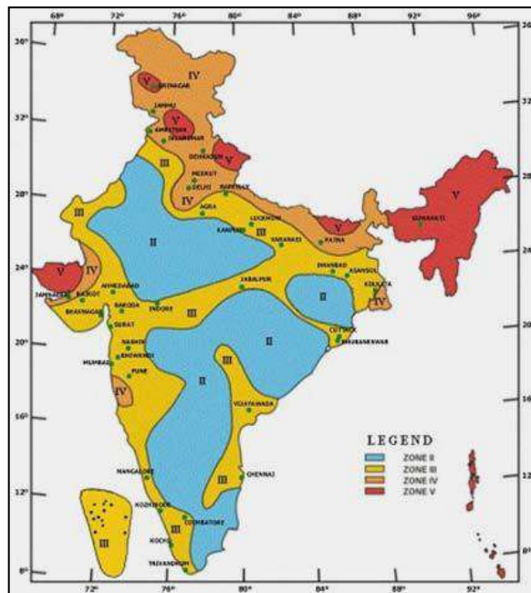
Figure 4.2 : Seismic Hazard Map showing Mumbai
