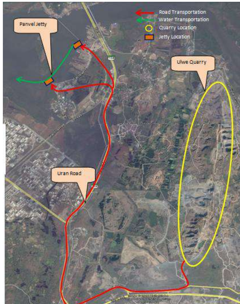
Figure 2.29: Transportation Plan from Ulwe Quarry
