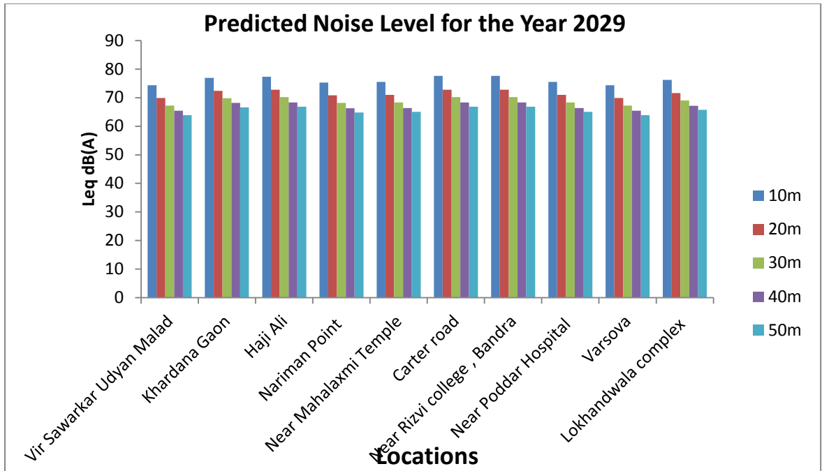
Figure 5.4: Noise prediction for the year 2029
