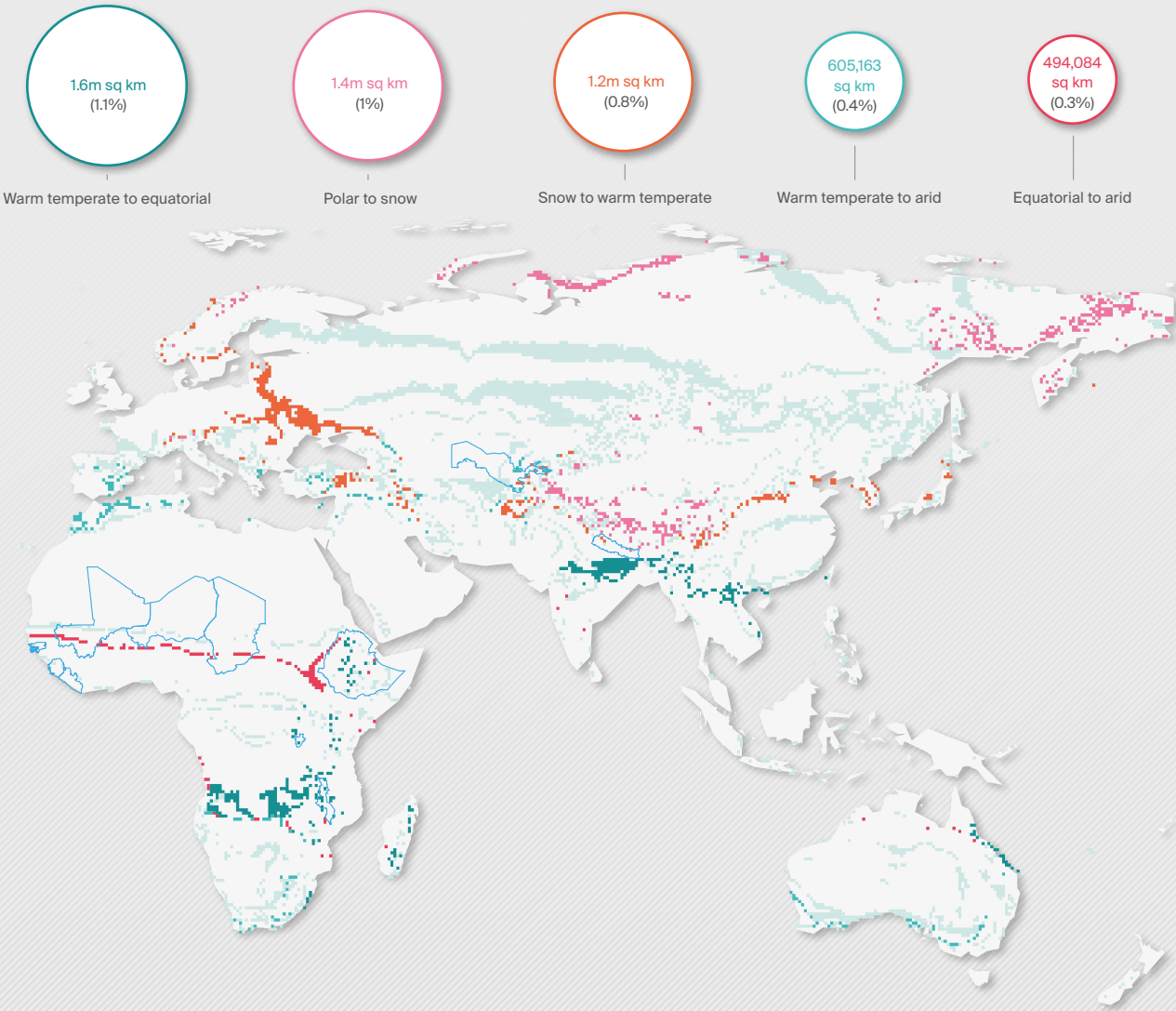
Area of the world's land mass affected by the five most significant climate shifts
