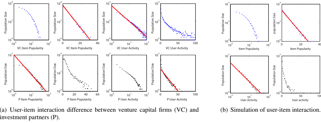
Figure 7.6: User-item Interaction Analysis.
