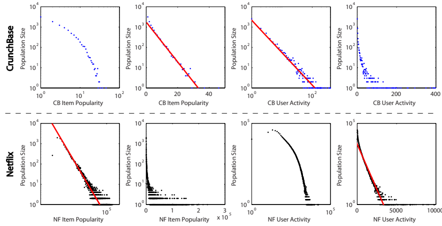
Figure 7.7: User-item Interaction for CrunchBase and Netflix.
