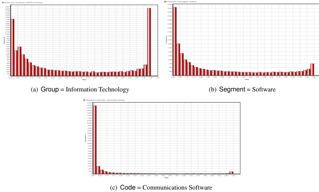
Figure 5.6: Example Distribution of Confidence Levels for Binary Class Membership of Group, Segment and Code.
