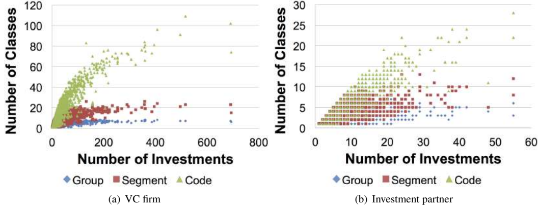
Figure 7.2: Number of Investments Against Number of Classes by User.
