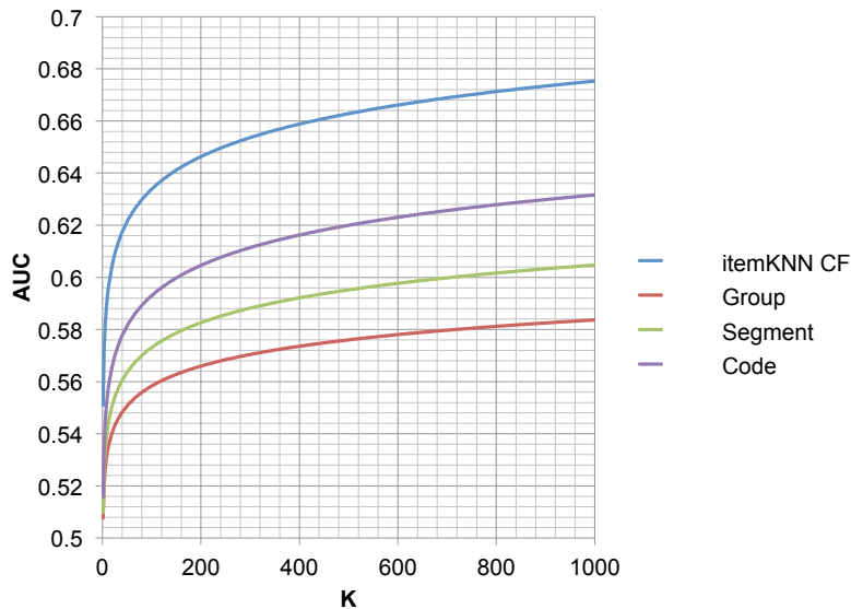
Figure 7.4: AUC Performance of Different Input Industry Classification Schemes Using k NN at Varying k on VentureSource dataset.
