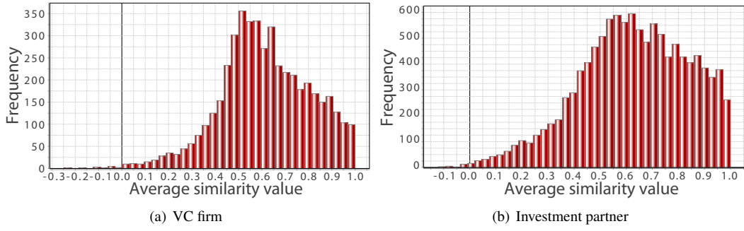
Figure 7.1: Average Pair-wise Cosine Similarity for VC and Investment Partner Portfolios.
