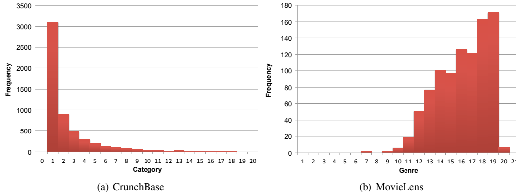
Figure 7.3: Unique Category Distribution by User.
