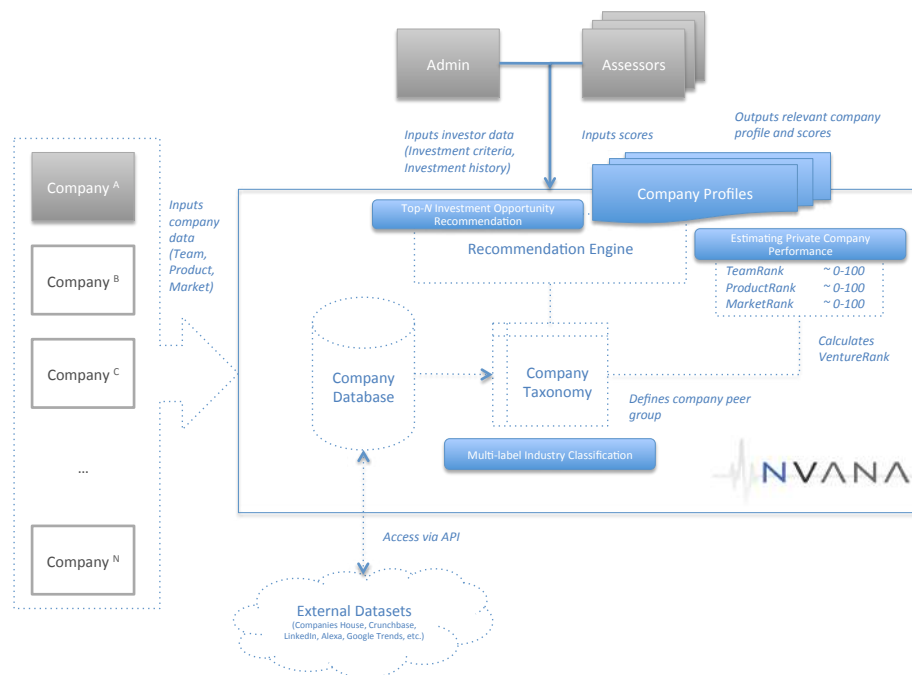
Figure 4.1: Overview of NVANA.
