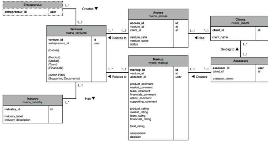
Figure 4.3: Entity Relationship (ER) Diagram for NVANA.
