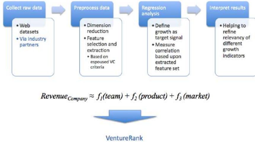
Figure 4.4: Proposed Process for Implementing VentureRank.
