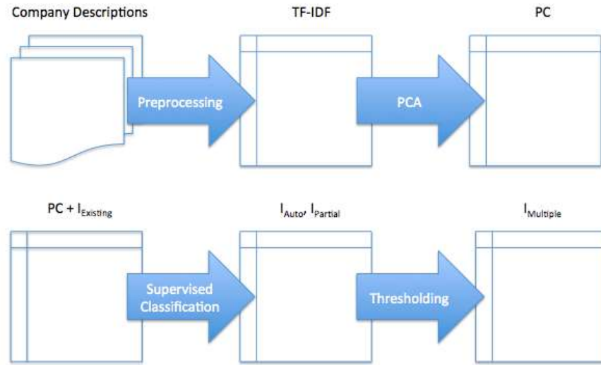
Figure 5.3: Process Diagram for Auto Classification and Multi-label Classification.
