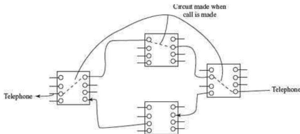
Figure 9.16 Circuit switching
