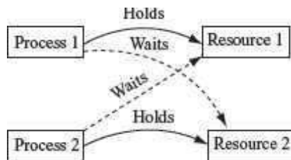
Figure 7.8 Deadlock
