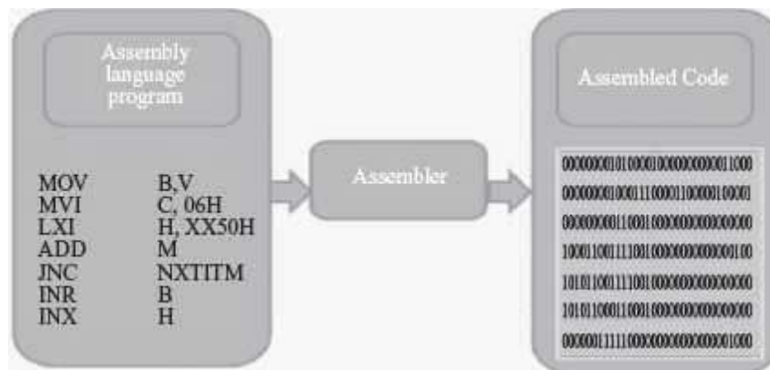
Figure 6.14 Assembler
